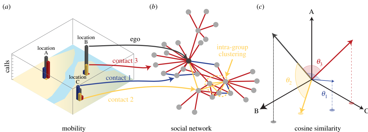
Figure 2. Similarity of visitation patterns between nodes in social networks. For each user, we keep track of (a) how many visits are made to locations across the city and (b) construct a social network by tracking calls to others. We can then define (c) the geographical cosine similarity between two users by computing the cosine of the angle between any two vectors in the location space.
